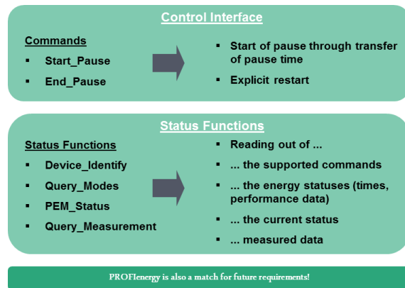
Fig. 26: PROFlenergy commands
