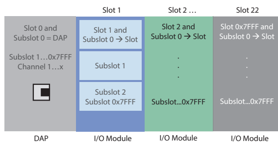
Fig. 3: Device model of a PROFINET field device
