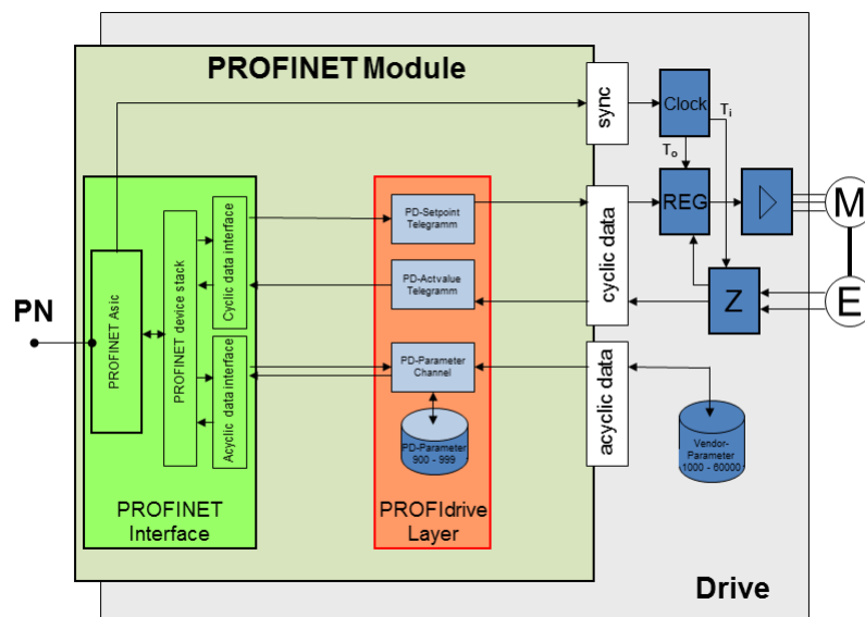
Fig. 25: PROFIdrive interface
