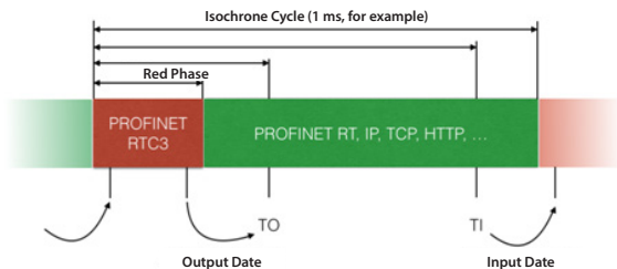
Fig. 5: Schematic representation of an isochronous cycle
