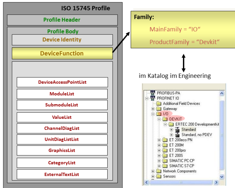
Fig. 19: Interaction between GSD and engineering
