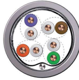
Fig. 7: Cross-section through an 8-wire PROFINET cable
